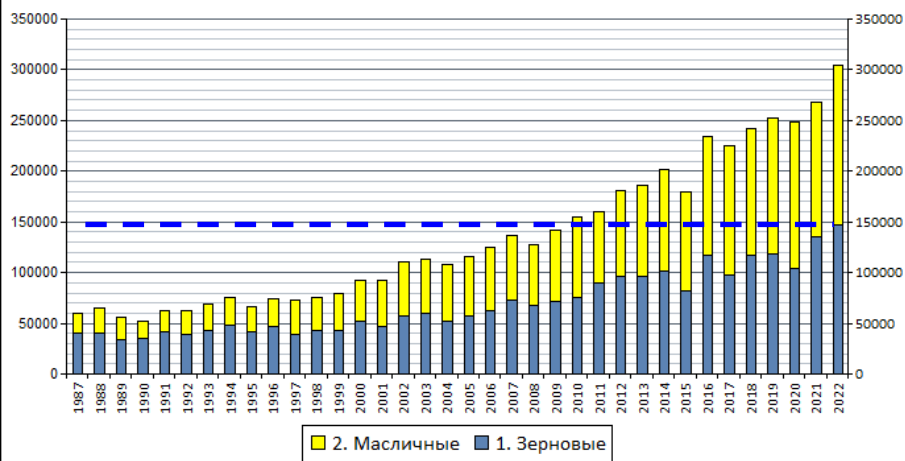
GO-SVCON-CONSUMP (RUB)
